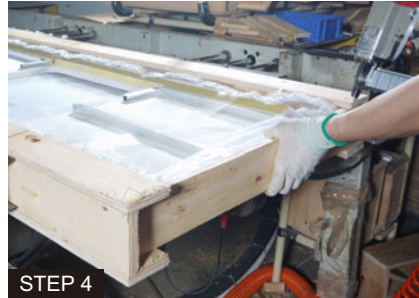
STEP 4 Nail the front plate.No exposure
