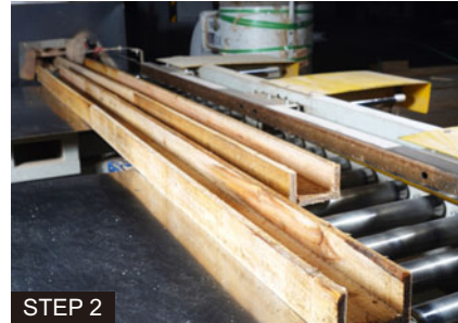
STEP 2 Cut the coaming following the countertop size
